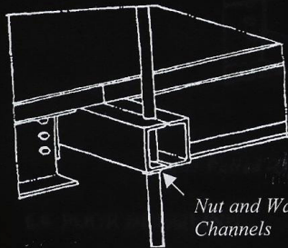
Fig. 5(a): Hyatt Regency Hanger Details As-Designed
